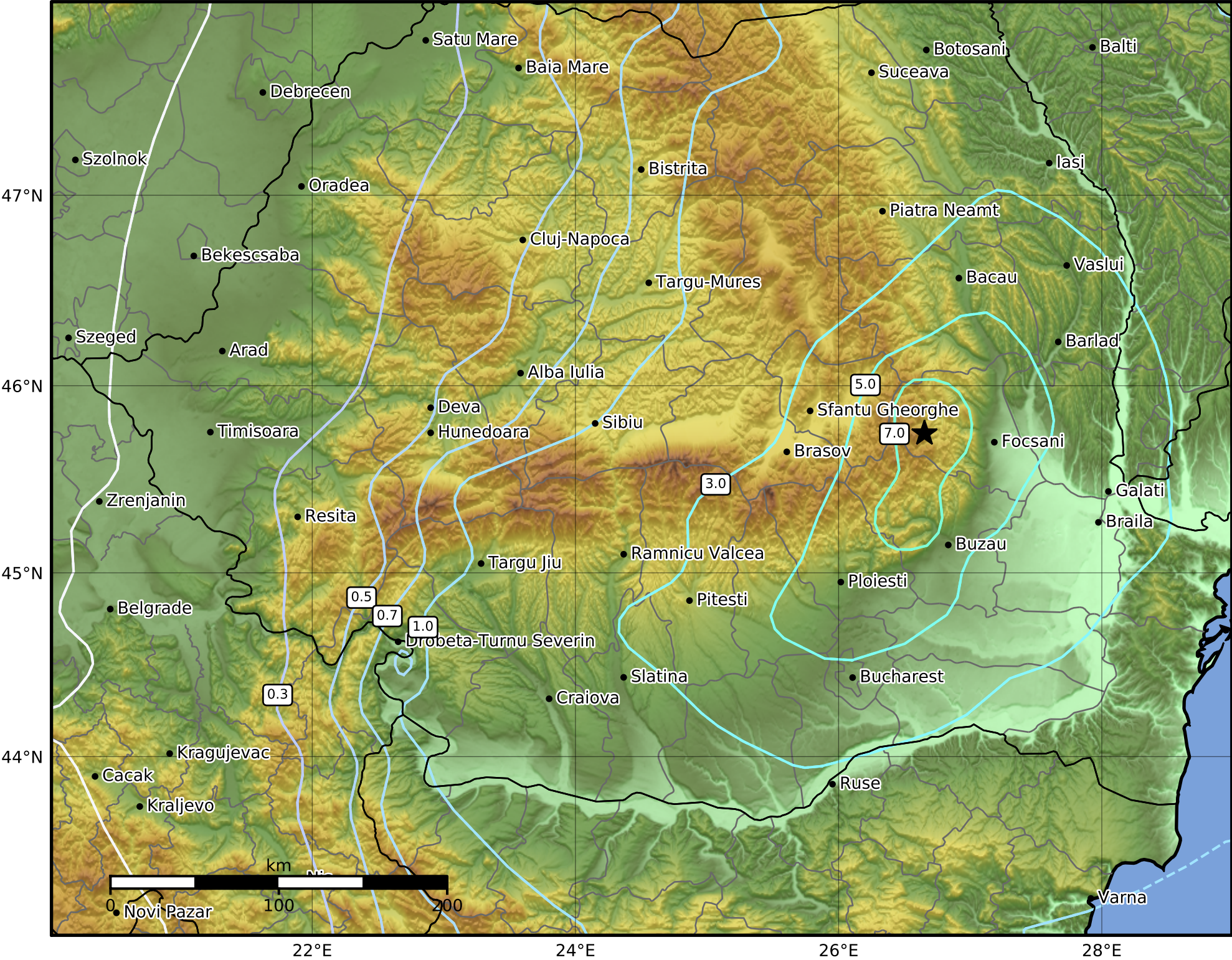
0.3 Second Peak Spectral Acceleration Map INFP ShakeMap: Vrancea EWS Romania Sep 23, 2016 23:11:16 UTC M5.8 N45.75 E26.65 Depth: 111.8km ID:202401
